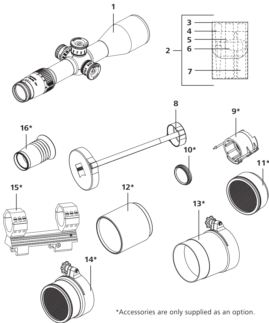
Illustration 1 Scope of Supply
